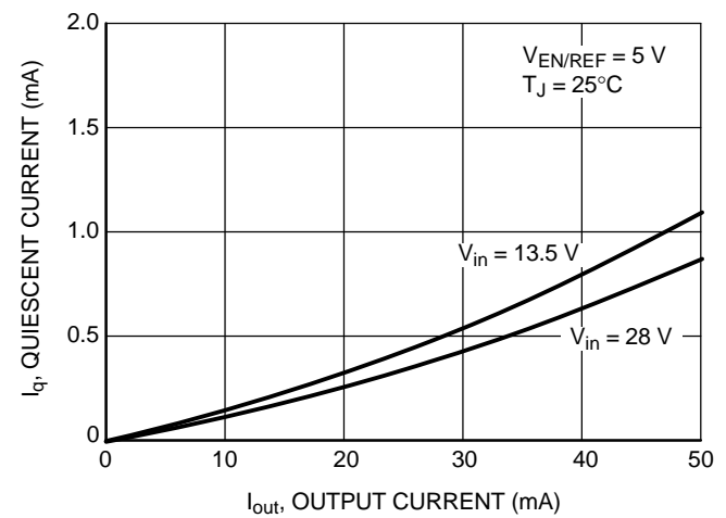
Figure 20. Current Consumption I_q vs. Output Current I_{out}
