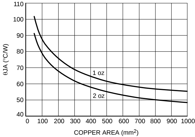
Figure 8. θ JA vs. Copper Spreader Area
