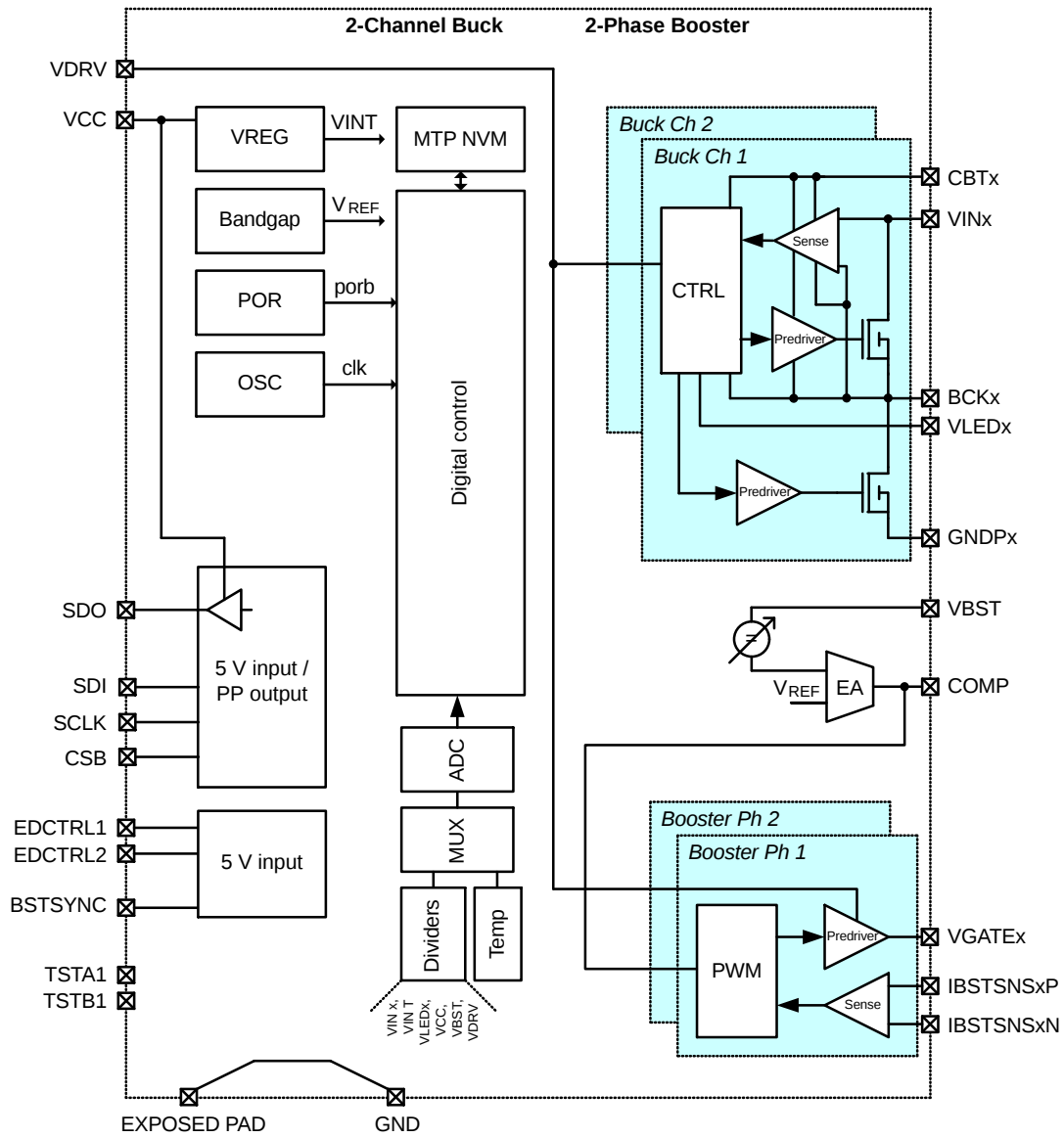
Figure 7. Block Diagram
