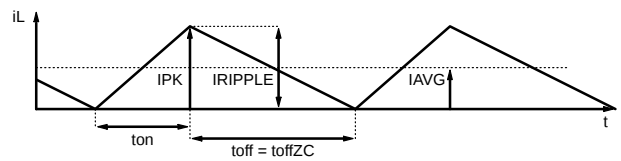
Figure 28. Inductor Current in BCM Mode
