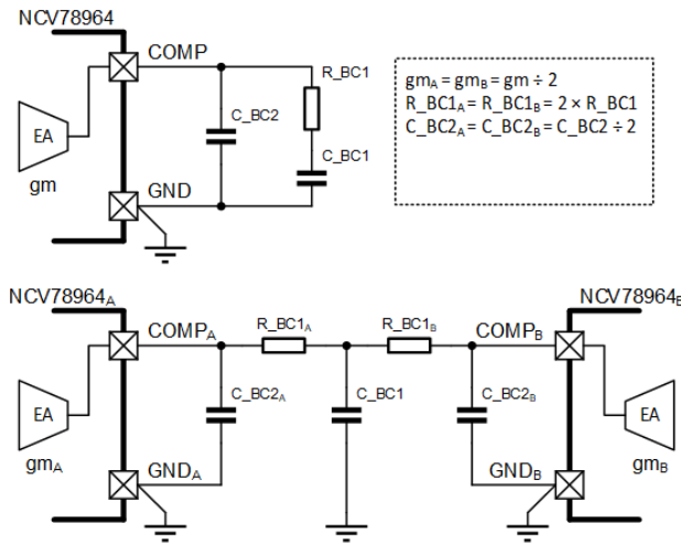
Figure 24. Compensation Network Connection for Single (Top) and Dual (Bottom) Device Operation
