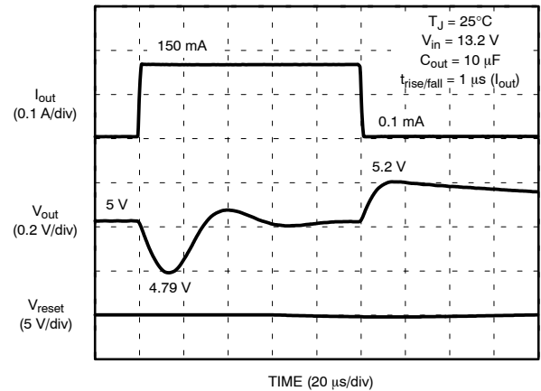
Figure 15. Load Transients
