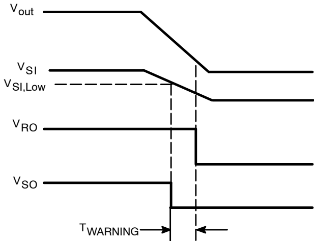
Figure 23. SO Warning Timing Diagram
