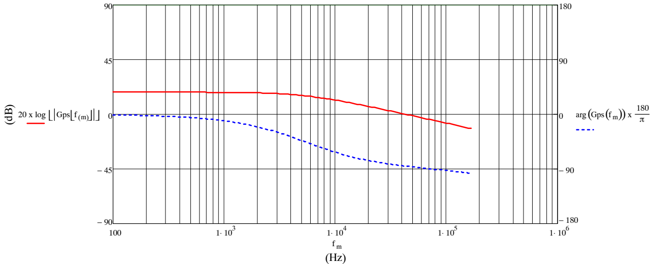
Figure 30. Power Stage Bode Plots
