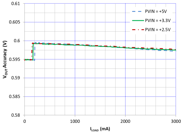
Figure 28. V_{OUT} Accuracy vs. I_{LOAD} and P_{VIN} V_{OUT} = 0.6\text{ V} , V_{AVIN} = 5.0\text{ V} , Auto Mode
