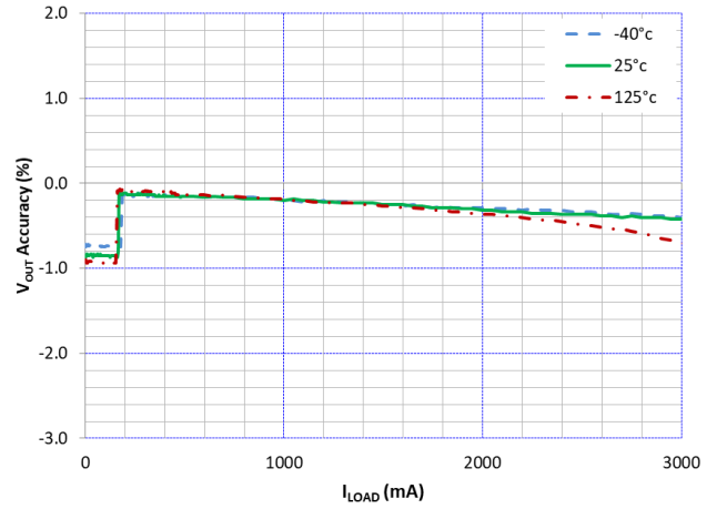
Figure 29. V_{OUT} Accuracy vs. I_{LOAD} and Temperature V_{OUT} = 0.6\text{ V} ; V_{AVIN} = 5.0\text{ V} , P_{VIN} = 3.3\text{ V} , Auto Mode
