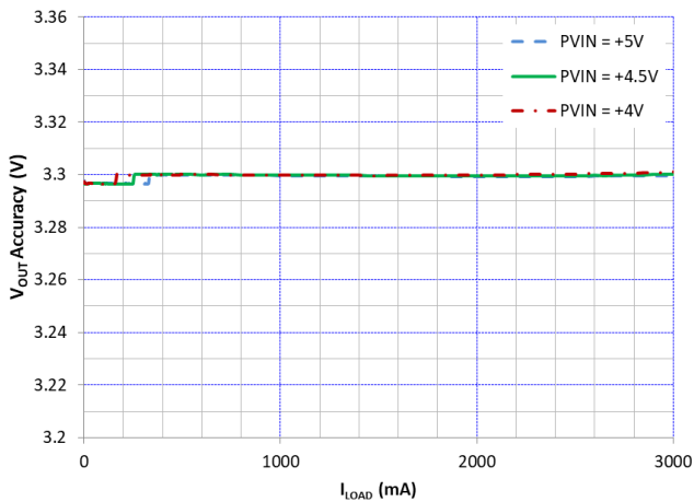
Figure 20. V_{OUT} Accuracy vs. I_{LOAD} and P_{VIN} V_{OUT} = 3.3\text{ V} , A_{VIN} = 5.0\text{ V} , Auto Mode
