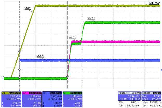
Figure 45. Switcher 2 Soft-start
