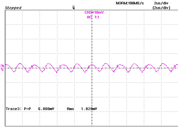
Figure 8: Output ripple & noise at 12Vin, 1.2V/50A out
