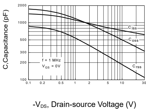
Figure 9: Capacitance Characteristics
