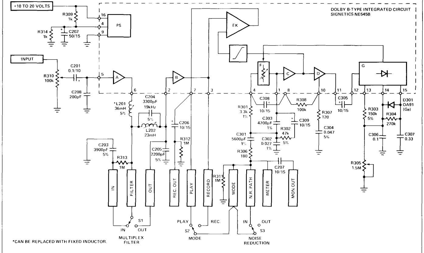
FIGURE 39. CLASS I PROCESSOR SHOWING CIRCUIT VARIATIONS
