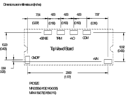
Recommended Pin Layout
