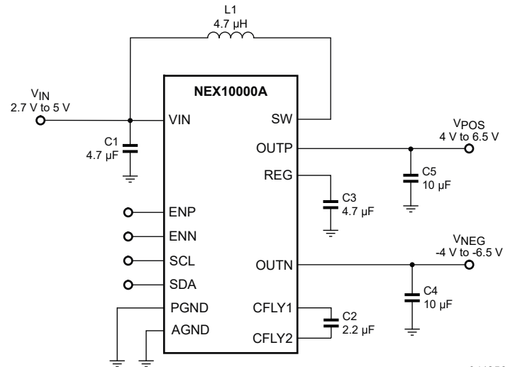
Fig. 1. Typical application
