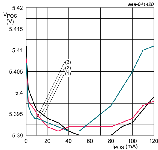
Fig. 18. V_{POS} versus positive output current (load regulation)
