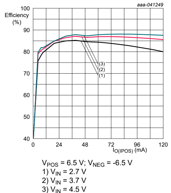
Fig. 2. Efficiency versus output current ( I_o )
