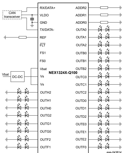
Fig. 1. Typical application
