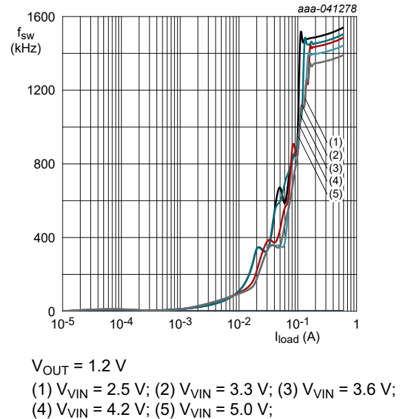
Fig. 26. Frequency versus load current
