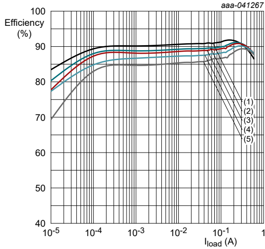
V_{OUT} = 1.3\text{ V} ; R_{SET} = 13.3\text{ k}\Omega ; L = 2.2\text{ }\mu\text{H} (1) V_{VIN} = 2.5\text{ V} ; (2) V_{VIN} = 3.3\text{ V} ; (3) V_{VIN} = 3.6\text{ V} ; (4) V_{VIN} = 4.2\text{ V} ; (5) V_{VIN} = 5.0\text{ V}
