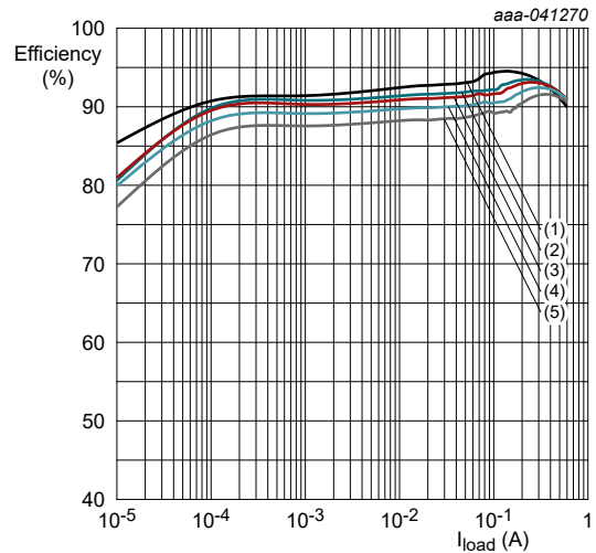
V_{OUT} = 1.85\text{ V} ; R_{SET} = 26.7\text{ k}\Omega ; L = 2.2\text{ }\mu\text{H} (1) V_{VIN} = 2.5\text{ V} ; (2) V_{VIN} = 3.3\text{ V} ; (3) V_{VIN} = 3.6\text{ V} ; (4) V_{VIN} = 4.2\text{ V} ; (5) V_{VIN} = 5.0\text{ V}
