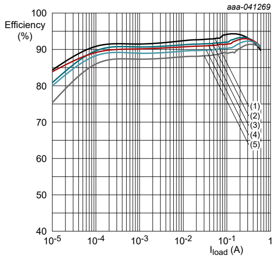
V_{OUT} = 1.8\text{ V} ; R_{SET} = 21.5\text{ k}\Omega ; L = 2.2\text{ }\mu\text{H} (1) V_{VIN} = 2.5\text{ V} ; (2) V_{VIN} = 3.3\text{ V} ; (3) V_{VIN} = 3.6\text{ V} ; (4) V_{VIN} = 4.2\text{ V} ; (5) V_{VIN} = 5.0\text{ V}
