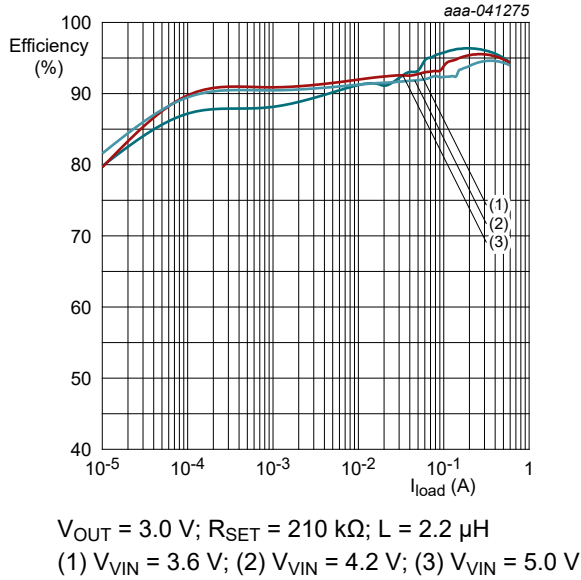
Fig. 23. Efficiency versus load current
