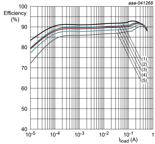
V_{OUT} = 1.5\text{ V} ; R_{SET} = 16.9\text{ k}\Omega ; L = 2.2\text{ }\mu\text{H} (1) V_{VIN} = 2.5\text{ V} ; (2) V_{VIN} = 3.3\text{ V} ; (3) V_{VIN} = 3.6\text{ V} ; (4) V_{VIN} = 4.2\text{ V} ; (5) V_{VIN} = 5.0\text{ V}
