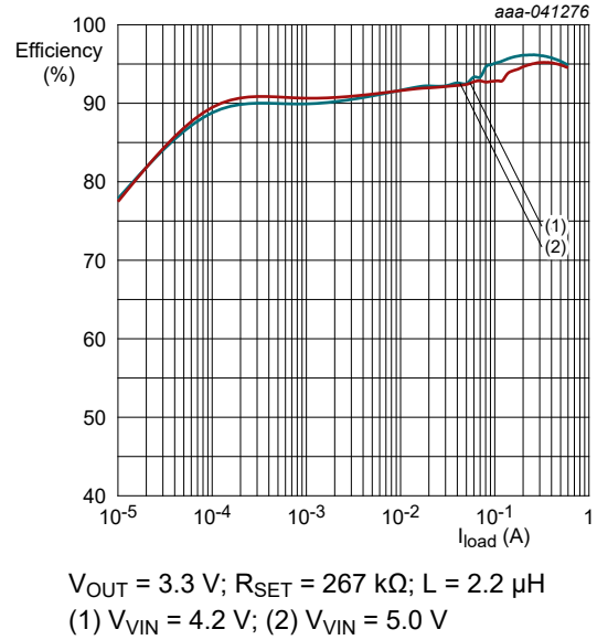
Fig. 24. Efficiency versus load current
