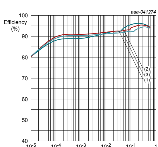
V_{OUT} = 2.95\text{ V} ; R_{SET} = 162\text{ k}\Omega ; L = 2.2\text{ }\mu\text{H} (1) V_{VIN} = 3.6\text{ V} ; (2) V_{VIN} = 4.2\text{ V} ; (3) V_{VIN} = 5.0\text{ V}
