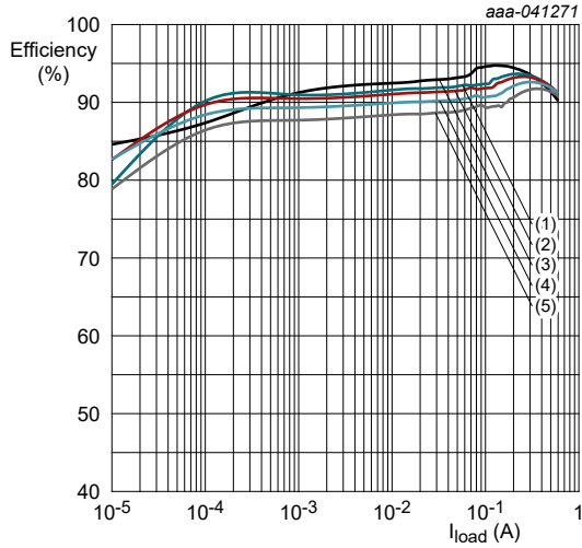
V_{OUT} = 1.9\text{ V} ; R_{SET} = 52.3\text{ k}\Omega ; L = 2.2\text{ }\mu\text{H} (1) V_{VIN} = 2.5\text{ V} ; (2) V_{VIN} = 3.3\text{ V} ; (3) V_{VIN} = 3.6\text{ V} ; (4) V_{VIN} = 4.2\text{ V} ; (5) V_{VIN} = 5.0\text{ V}
