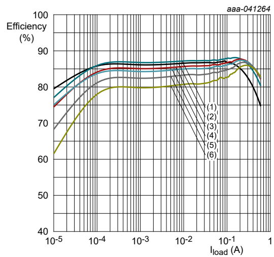
V_{OUT} = 0.8\text{ V} ; R_{SET} = 5.11\text{ k}\Omega ; L = 2.2\text{ }\mu\text{H} (1) V_{VIN} = 1.8\text{ V} ; (2) V_{VIN} = 2.5\text{ V} ; (3) V_{VIN} = 3.3\text{ V} ; (4) V_{VIN} = 3.6\text{ V} ; (5) V_{VIN} = 4.2\text{ V} ; (6) V_{VIN} = 5.0\text{ V}
