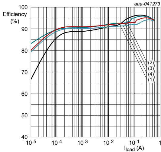
V_{OUT} = 2.8\text{ V} ; R_{SET} = 118\text{ k}\Omega ; L = 2.2\text{ }\mu\text{H} (1) V_{VIN} = 3.3\text{ V} ; (2) V_{VIN} = 3.6\text{ V} ; (3) V_{VIN} = 4.2\text{ V} ; (4) V_{VIN} = 5.0\text{ V}
