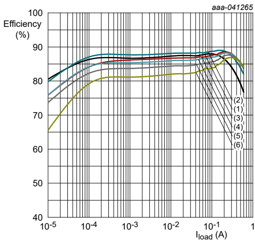
V_{OUT} = 0.9\text{ V} ; R_{SET} = 7.5\text{ k}\Omega ; L = 2.2\text{ }\mu\text{H} (1) V_{VIN} = 1.8\text{ V} ; (2) V_{VIN} = 2.5\text{ V} ; (3) V_{VIN} = 3.3\text{ V} ; (4) V_{VIN} = 3.6\text{ V} ; (5) V_{VIN} = 4.2\text{ V} ; (6) V_{VIN} = 5.0\text{ V}
