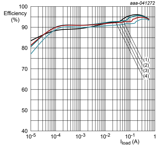
V_{OUT} = 2.7\text{ V} ; R_{SET} = 82.5\text{ k}\Omega ; L = 2.2\text{ }\mu\text{H} (1) V_{VIN} = 3.3\text{ V} ; (2) V_{VIN} = 3.6\text{ V} ; (3) V_{VIN} = 4.2\text{ V} ; (4) V_{VIN} = 5.0\text{ V}
