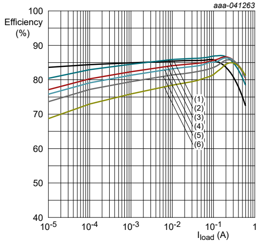
V_{OUT} = 0.7\text{ V} ; R_{SET} = 3.32\text{ k}\Omega ; L = 2.2\text{ }\mu\text{H} (1) V_{VIN} = 1.8\text{ V} ; (2) V_{VIN} = 2.5\text{ V} ; (3) V_{VIN} = 3.3\text{ V} ; (4) V_{VIN} = 3.6\text{ V} ; (5) V_{VIN} = 4.2\text{ V} ; (6) V_{VIN} = 5.0\text{ V}
