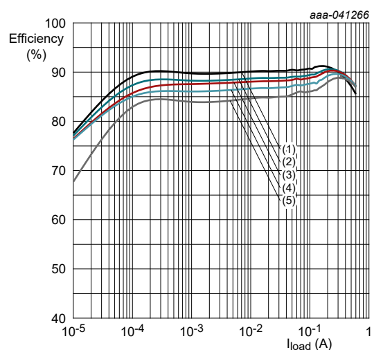
V_{OUT} = 1.2\text{ V} ; R_{SET} = 10.2\text{ k}\Omega ; L = 2.2\text{ }\mu\text{H} (1) V_{VIN} = 2.5\text{ V} ; (2) V_{VIN} = 3.3\text{ V} ; (3) V_{VIN} = 3.6\text{ V} ; (4) V_{VIN} = 4.2\text{ V} ; (5) V_{VIN} = 5.0\text{ V}
