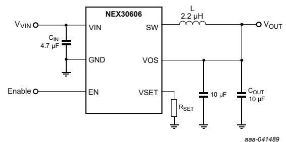
Fig. 1. Typical application
