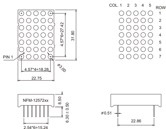
NFM-12572 Series
