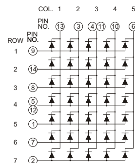
NFM-12573Bx
