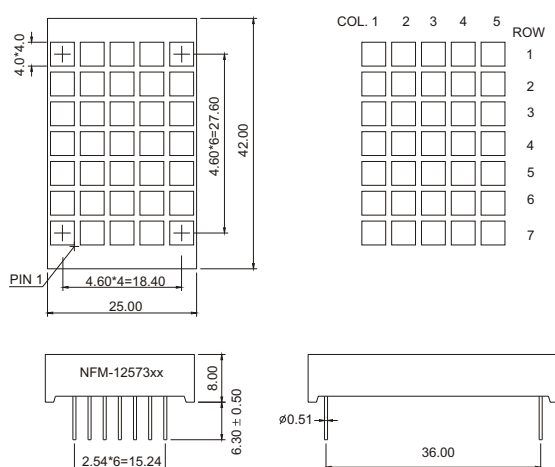
NFM-12573 Series
