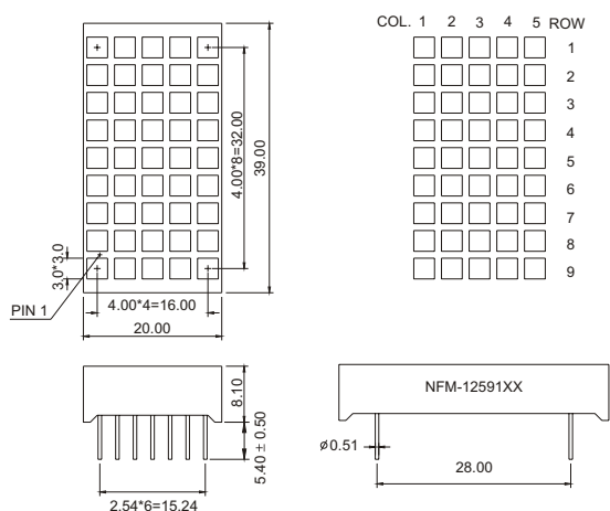
NFM-12591 Series
