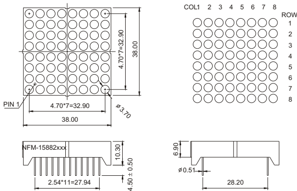
NFM-15882 Series
