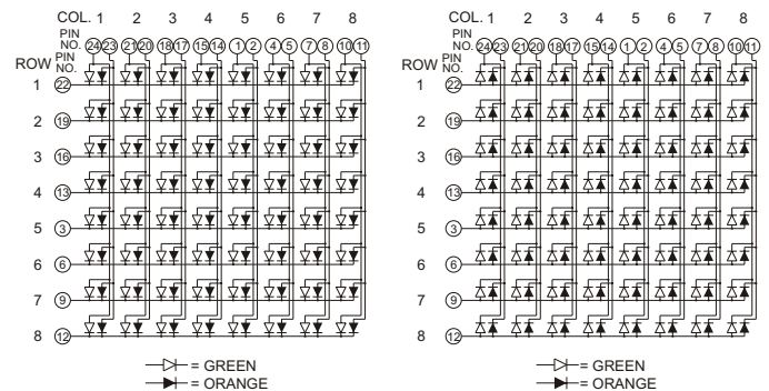
NFM-15882CEG
