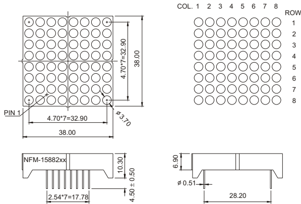
NFM-15882 Series
