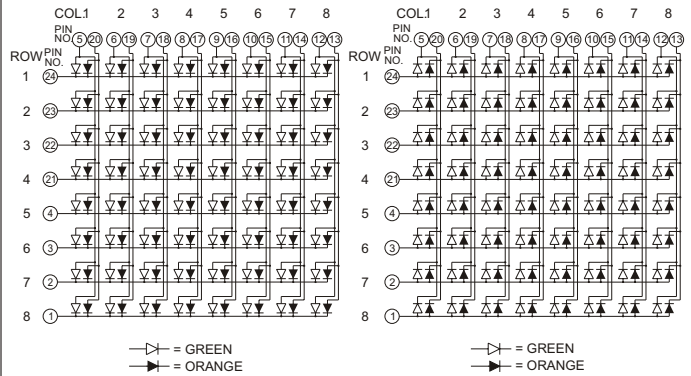
NFM-15882AEG
