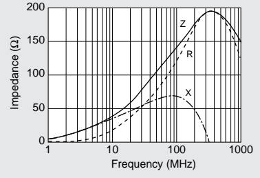
BLM10A102SG
