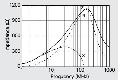
BLM10A102SG
