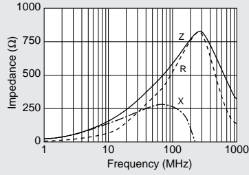
BLM10A601SG
