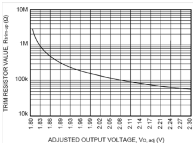
Figure 24. NH020Y Rtrim-up Test Results.
