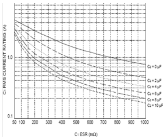
Figure 19. Electrolytic Capacitor ESR and RMS Current Rating Data.
