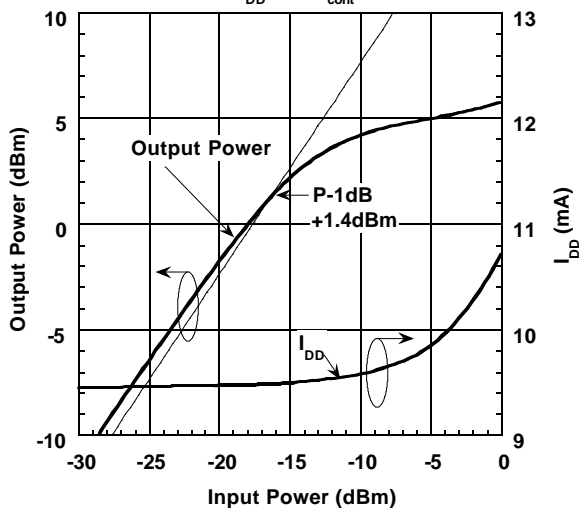
OUTPUT POWER, I_{DD} vs. INPUT POWER ( V_{DD} = 3V, V_{cont} = 2V, f = 1.5GHz )
