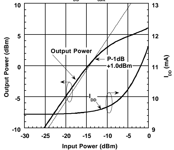
OUTPUT POWER, I_{DD} vs. INPUT POWER ( V_{DD} = 3V, V_{cont} = 2V, f = 2.5GHz )
