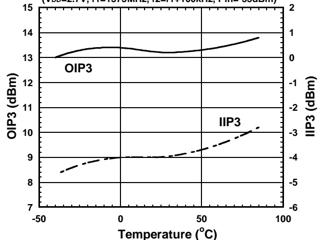
OIP3, IIP3 vs. Temperature
