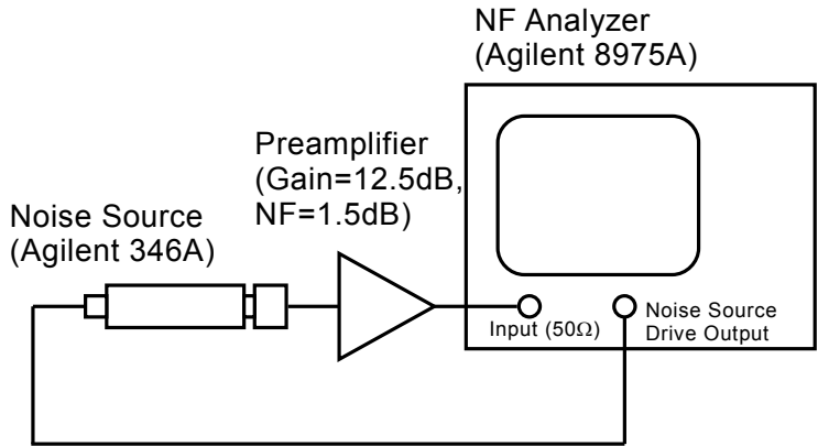
Calibration Setup
