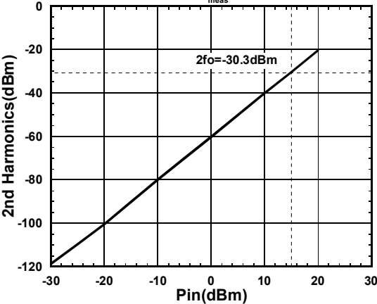
2nd Harmonics
