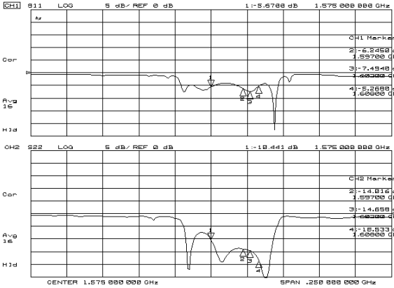
S11, S22
