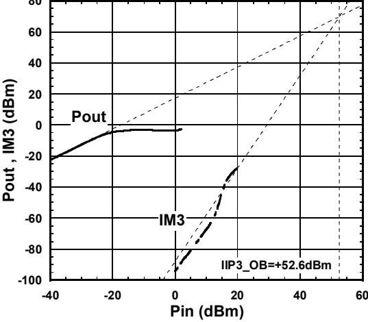
Out-of-band IIP3
