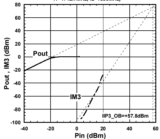
Out-of-band IIP3
