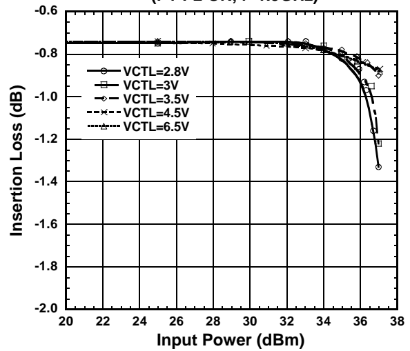
Insertion Loss vs. Input Power (P1-P2 ON, f=1.9GHz)
