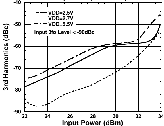
3rd Harmonics vs. Input Power ( f=2GHz, PC-P1on )
