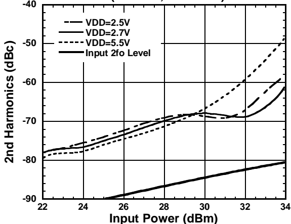
2nd Harmonics vs. Input Power ( f=2GHz, PC-P1on )
