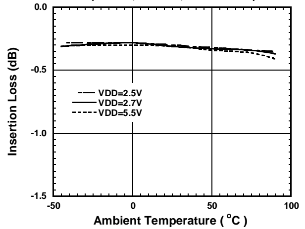
Loss vs. Ambient Temperature
