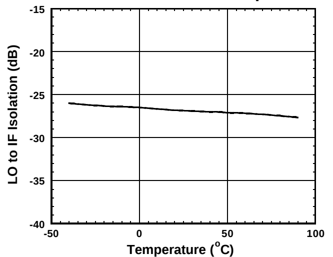
LO to IF Isolation vs. Temperature
