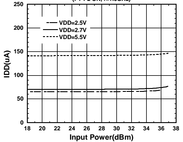
IDD vs. Input Power (P1-P2 ON, f=1.9GHz)
