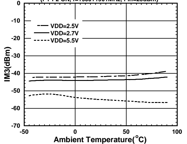
IM3 vs. Ambient Temperature
