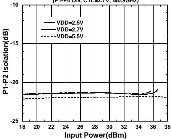
Isolation vs. Input Power (P1-P4 ON, CTL=2.7V, f=0.9GHz)
