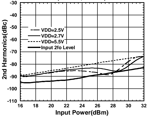
2nd Harmonics vs. Input Power (P1-P2 ON, f=0.9GHz)
