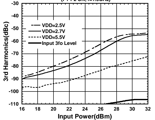
3rd Harmonics vs. Input Power (P1-P2 ON, f=1.9GHz)
