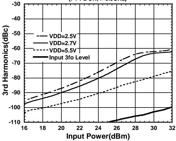
3rd Harmonics vs. Input Power (P1-P2 ON, f=0.9GHz)
