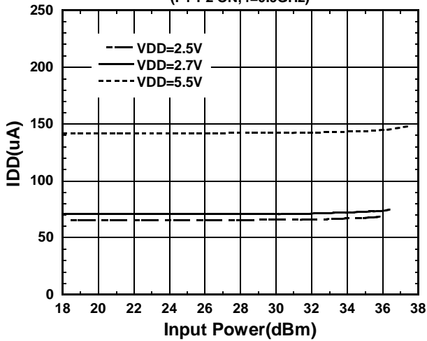
IDD vs. Input Power (P1-P2 ON, f=0.9GHz)
