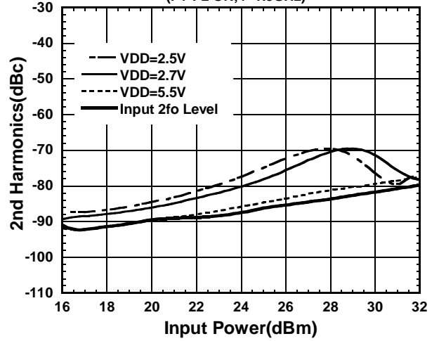
2nd Harmonics vs. Input Power (P1-P2 ON, f=1.9GHz)
