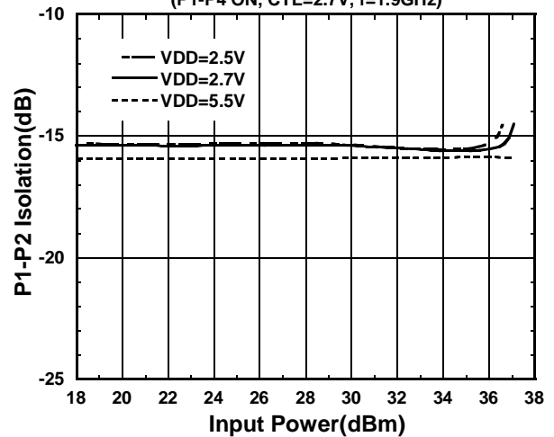
Isolation vs. Input Power (P1-P4 ON, CTL=2.7V, f=1.9GHz)
