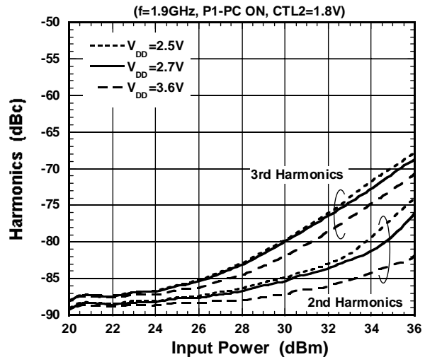
Harmonics vs Input Power ( f=1.9\text{GHz} , P1-PC ON, CTL2=1.8V)
