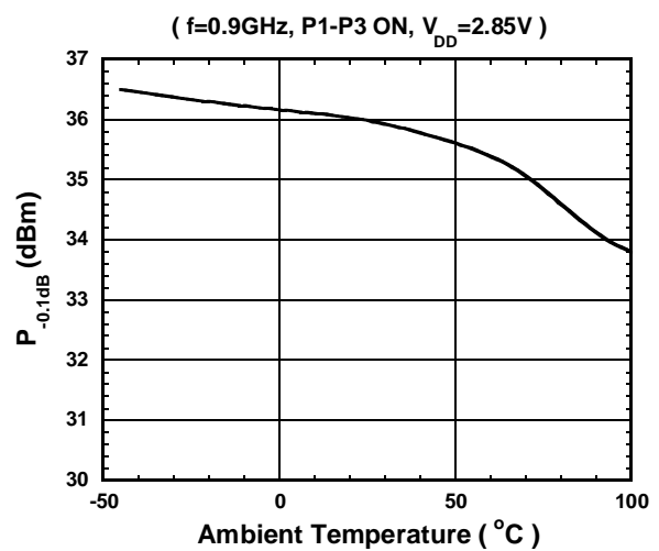
P -0.1dB vs. Ambient Temperature
