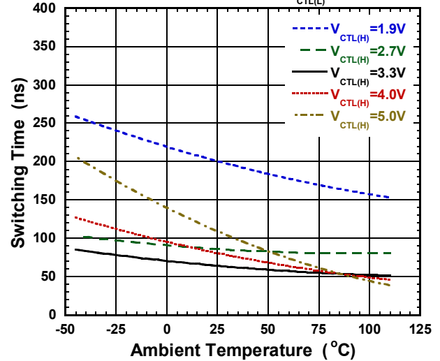
Switching Time(rise) vs Temperature
