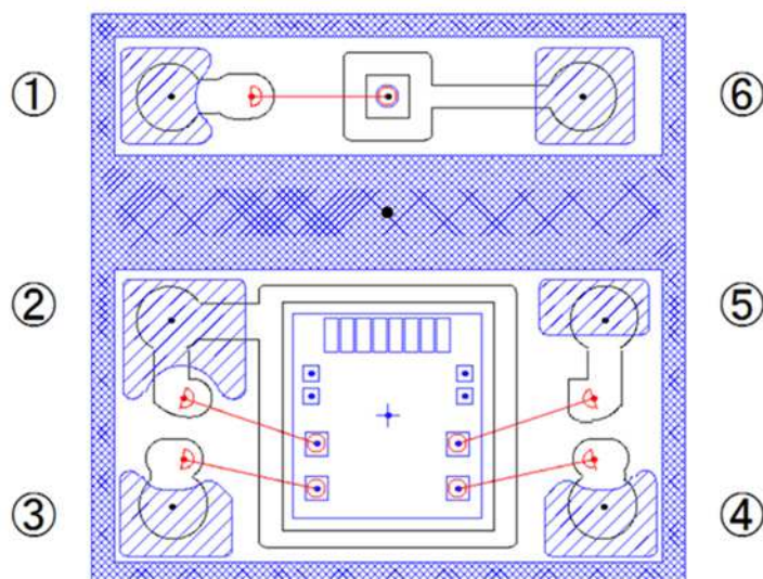
Pin Configuration
