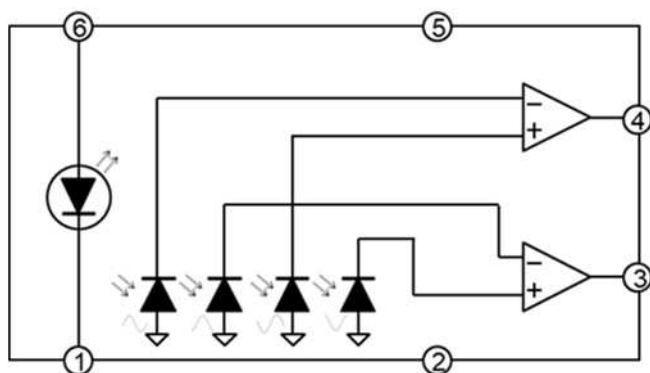
NJL5821/22R Block Diagram
