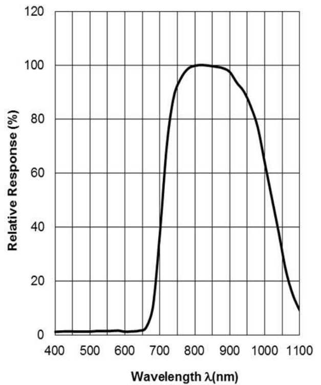
Spectral Response (Ta=25°C)
