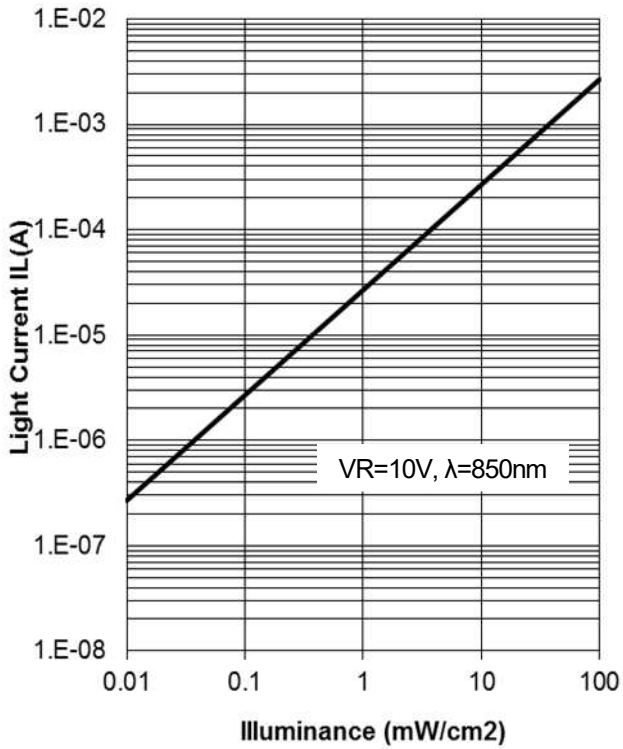
Light Current vs. Illuminance (Ta=25°C)
