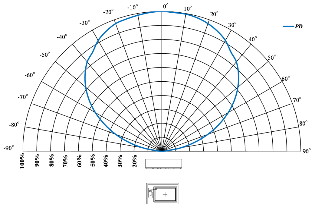
Directivity at Package direction Y
