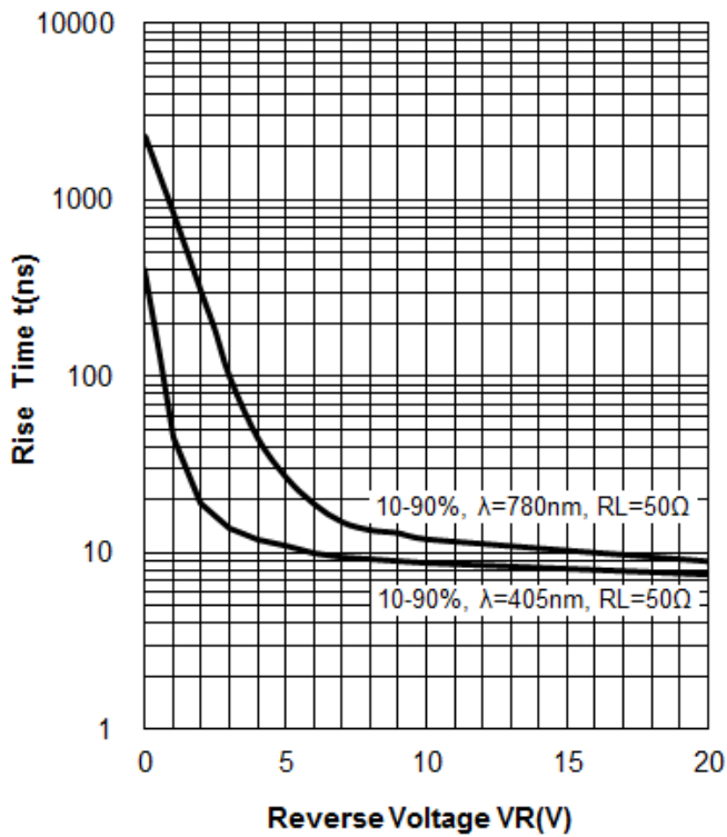
Rise time vs. Reverse Voltage (Ta=25°C)
