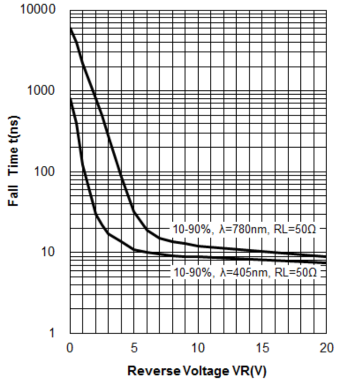
Fall time vs. Reverse Voltage (Ta=25°C)
