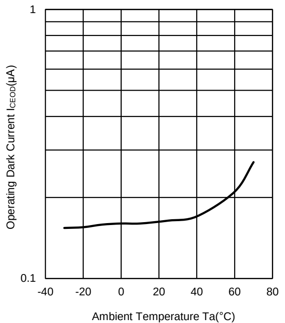
Operating Dark Current vs. Temperature I_F = 5\text{mA}, V_{CE0} = 3.3\text{V}
