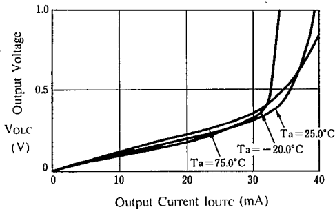
Output Voltage (OUTc) vs. Output Current (Iourc)
