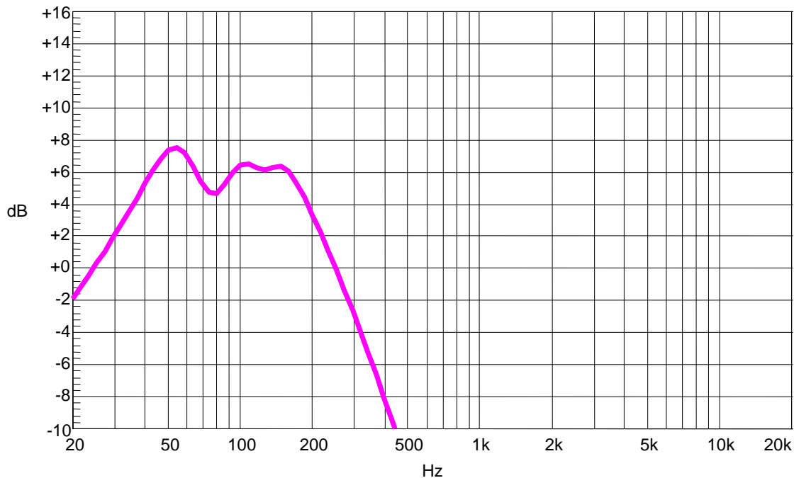
NJM2192A(TruBass) GAIN STRUCTURE "Speaker Size : Medium"
