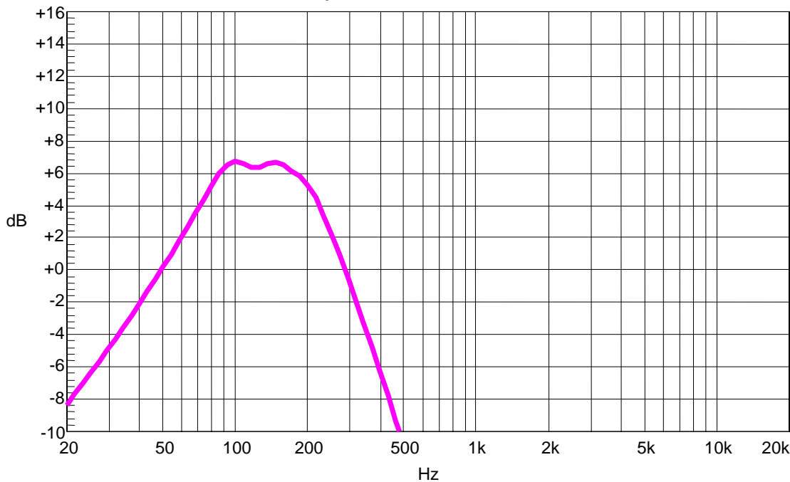
NJM2192A(TruBass) GAIN STRUCTURE "Speaker Size : Small"
