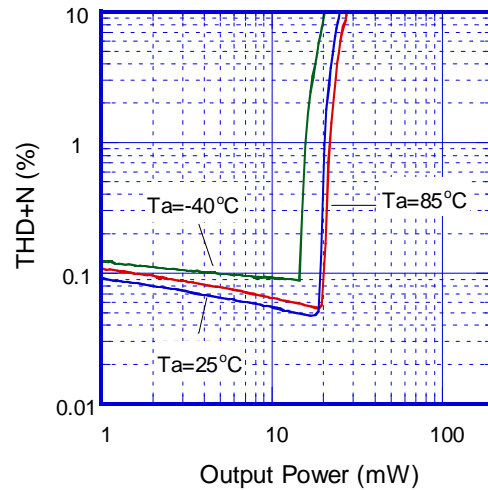
THD+N vs. Output Power ( V_+ = 2.8V, f = 1KHz, R_L = 16\Omega )
