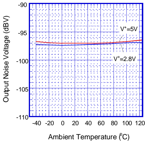
Output Noise Voltage vs. Ambient Temperature ( R_L = 32\Omega, A -Weighed)
