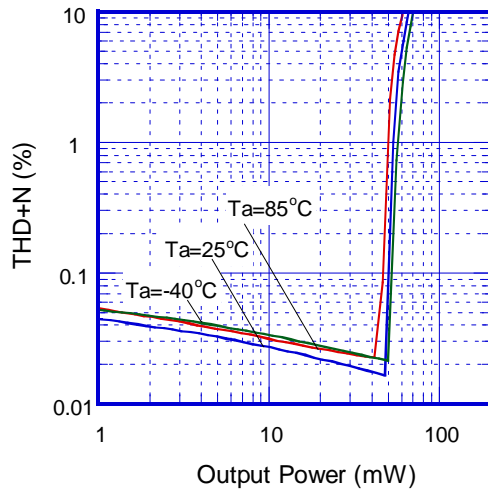
THD+N vs. Output Power ( V_+ = 5V, f = 1KHz, R_L = 32\Omega )
