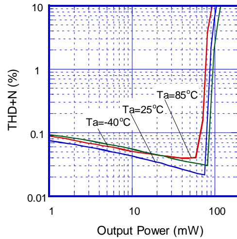
THD+N vs. Output Power ( V_+ = 5V, f = 1KHz, R_L = 16\Omega )
