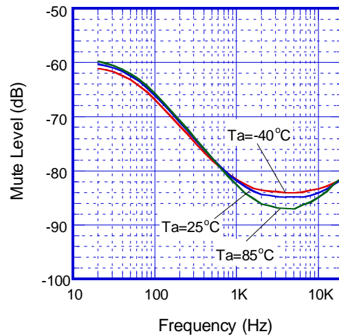
Mute Level vs. Frequency ( V_+ = 5V, V_{in} = -6dBV, R_L = 32\Omega )
