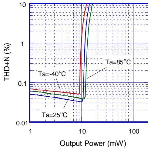
THD+N vs. Output Power ( V_+ = 2.8V, f = 1KHz, R_L = 32\Omega )
