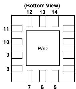
NJM2903CMD7 (Note1, 2, 3)
