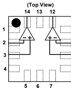
NJM2903CMD7 (Note1, 2, 3)
