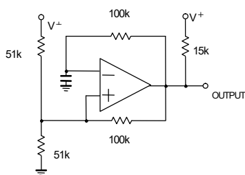
Pulse Generator
