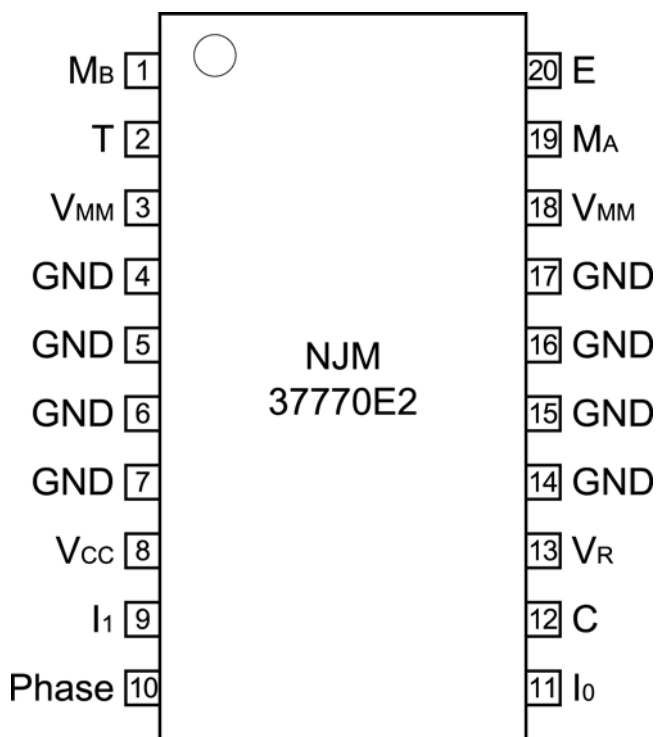
Figure 2. Pin configuration
