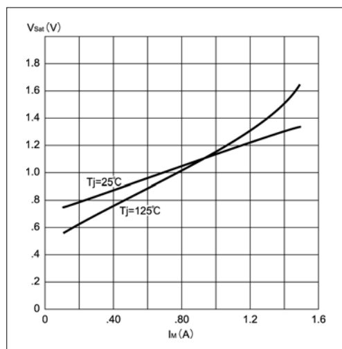
Figure 10. Typical source saturation vs. output current
