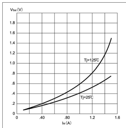
Figure 12. Typical sink saturation vs. output current
