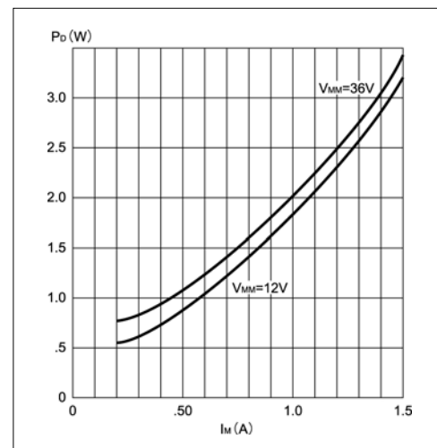
Figure 13. Typical power dissipation vs. motor current
