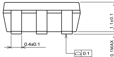
SOT-23-5Package
