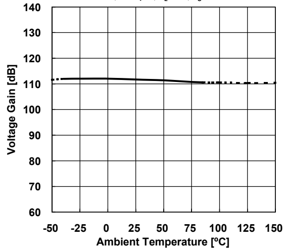
Open Loop Gain vs. Temperature V^+/V^-=\pm 15V, G_v=open, R_l=2k\Omega, V_o=-10V to +10V
