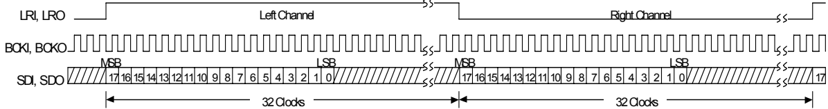
Fig.5-8 Left-Justified Data Format 64fs, 18bit Data
