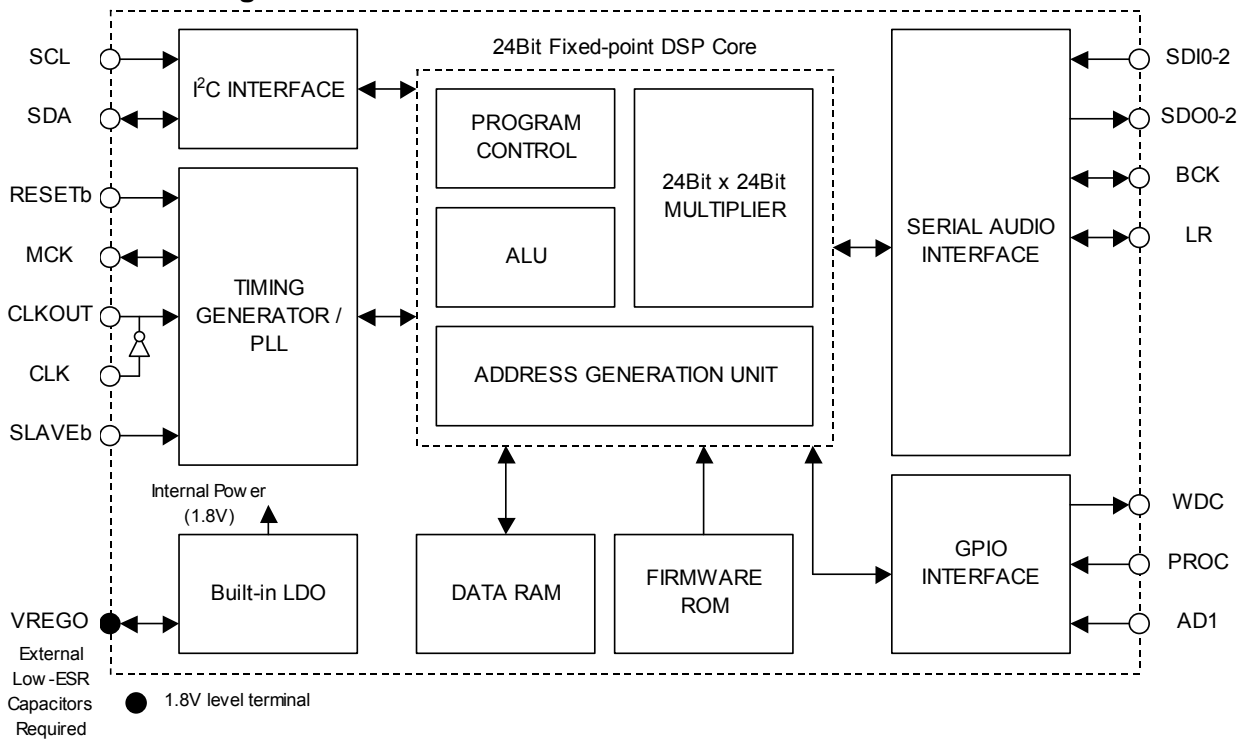
Fig. 1 NJU26126 Block Diagram
