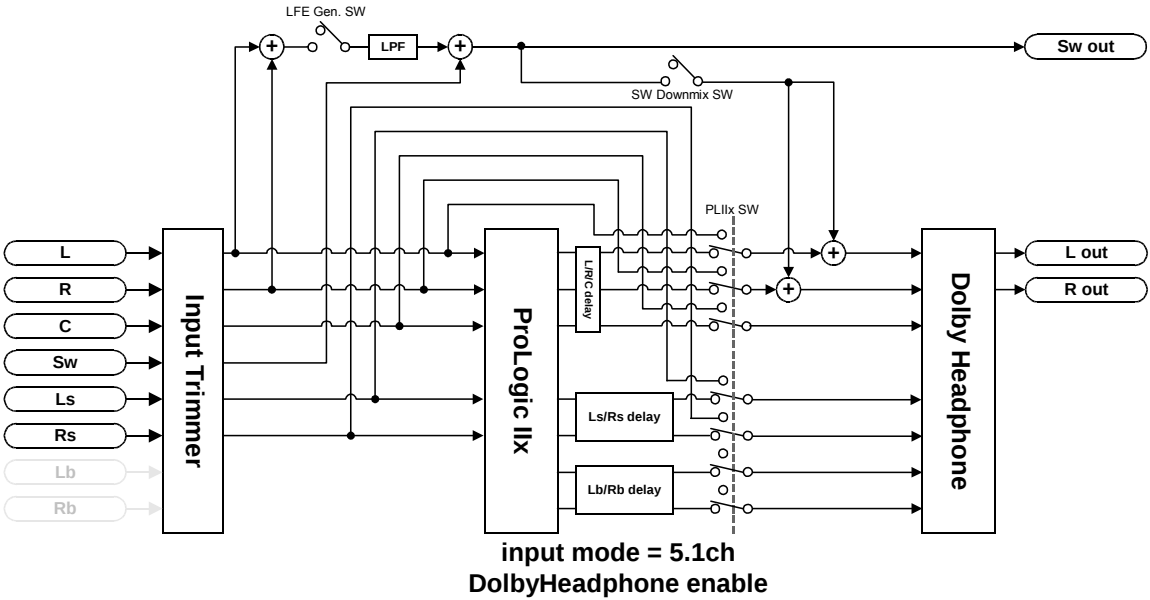
Fig. 2.4 NJU26226 Block Diagram (detail)
