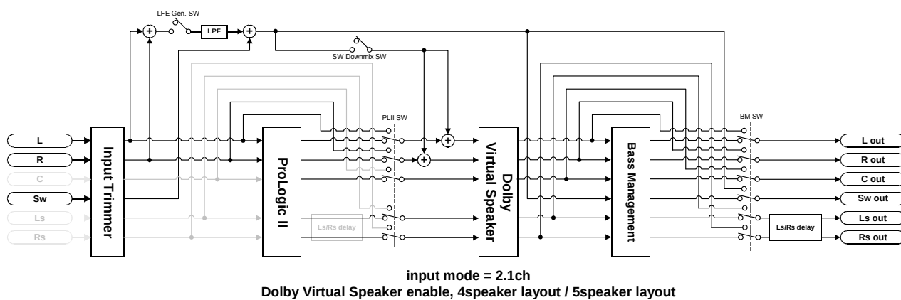
Fig. 2.10 NJU26226 Block Diagram (detail)
