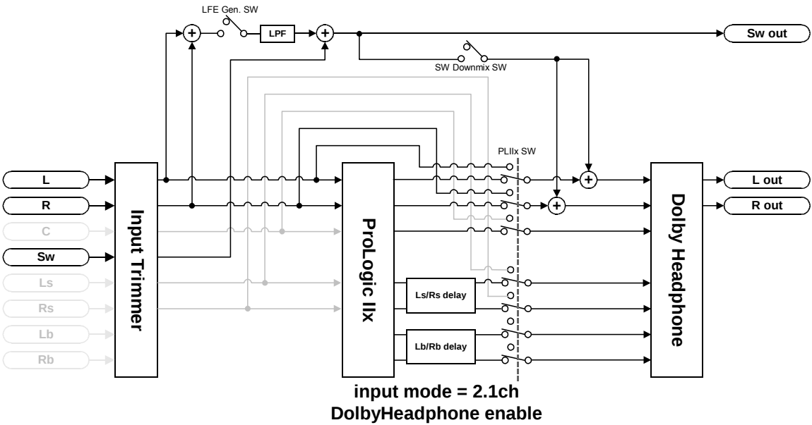
Fig. 2.3 NJU26226 Block Diagram (detail)
