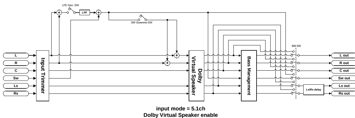
Fig. 2.11 NJU26226 Block Diagram (detail)
