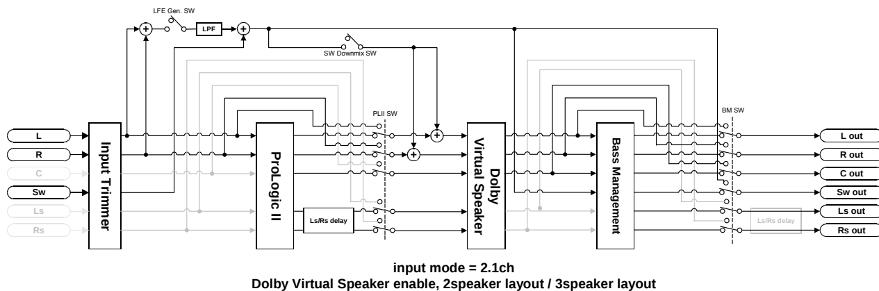
Fig. 2.9 NJU26226 Block Diagram (detail)
