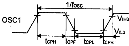
EXTERNAL CLOCK
