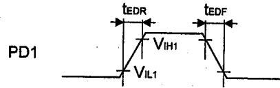
RESTART SIGNAL INPUT
