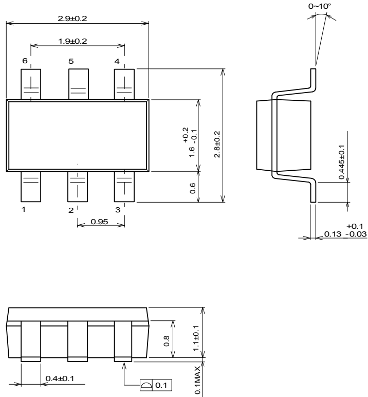
SOT-23-6-1 Package
