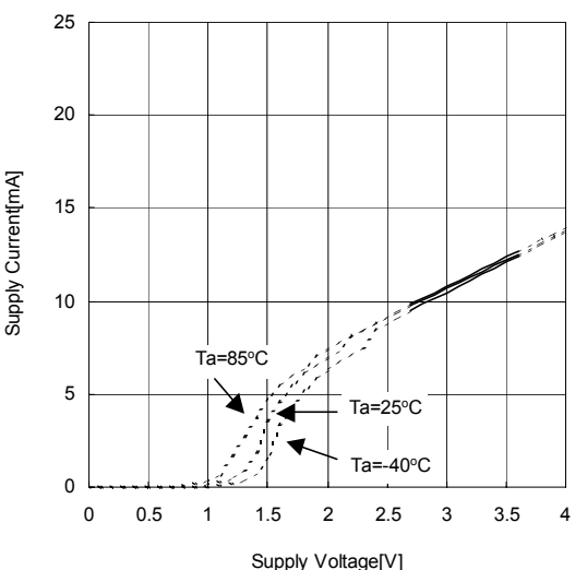
Supply Current vs Supply Voltage RL=NoLoad, MUTE=H, GAIN=H
