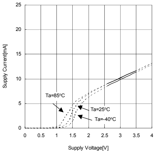
Supply Current vs Supply Voltage RL=NoLoad, MUTE=L, GAIN=H
