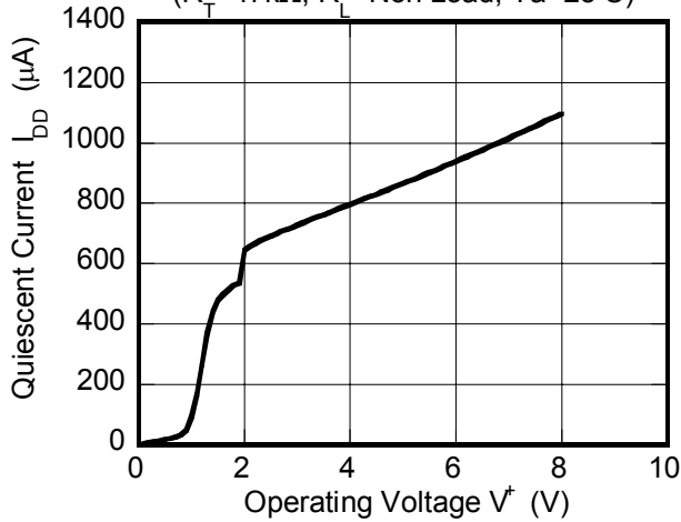
Quiescent Current vs. Operating Voltage (R T =47kΩ, R L =Non Load, Ta=25°C)
