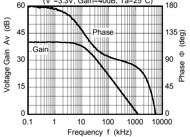
Error Amplifier Block Voltage Gain, Phase vs. Frequency (V + =3.3V, Gain=40dB, Ta=25°C)
