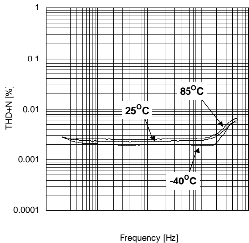
THD+N vs. Frequency V_{\pm}=\pm 7V , V_{in}=2Vrms , TONE=ON, BW:10-80kHz
