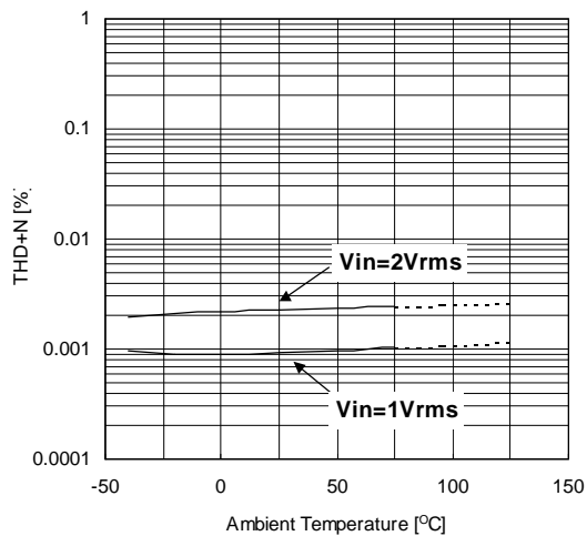
THD+N vs. Ambient Temperature V_{\pm}=\pm 7V , f=1kHz , TONE=ON, BW:400-30kHz
