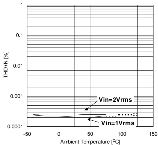
THD+N vs. Ambient Temperature V_{\pm}=\pm 7V , f=1kHz , TONE=OFF, BW:400-30kHz
